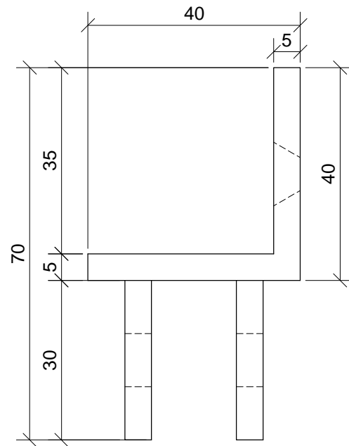
PLAN VIEW
