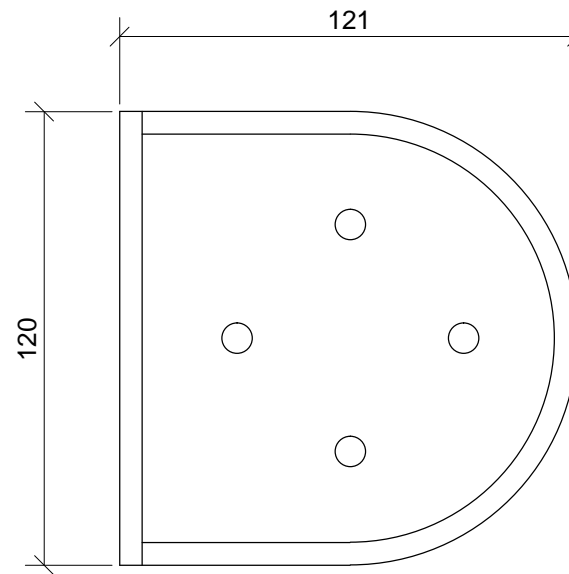
RHS Bracket SIDE PROFILE
